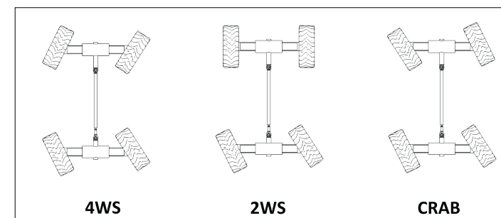
Steering System
